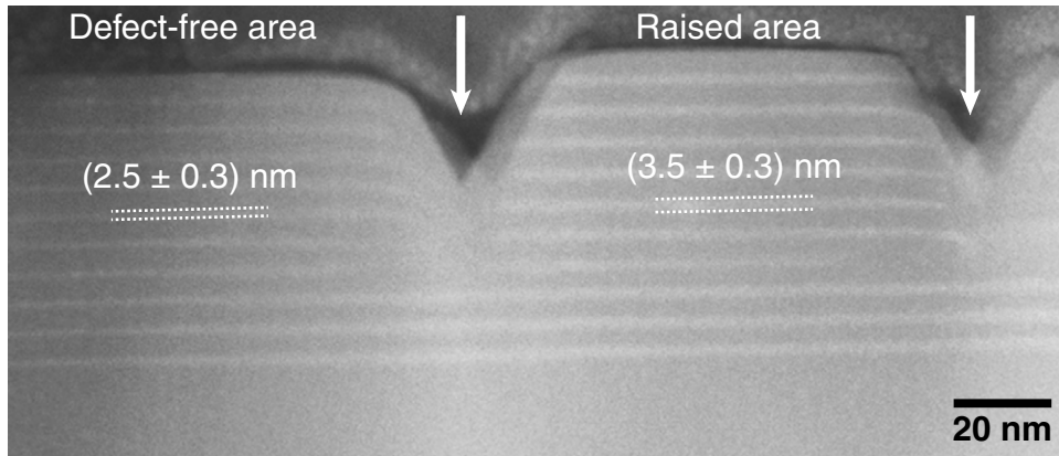
Figure 4. HAADF image of a sectioned raised trench defect of a ten-period InGaN/GaN MQW structure, with trenches indicated by arrows. The thickness of the InGaN QWs is indicated by dotted lines.
