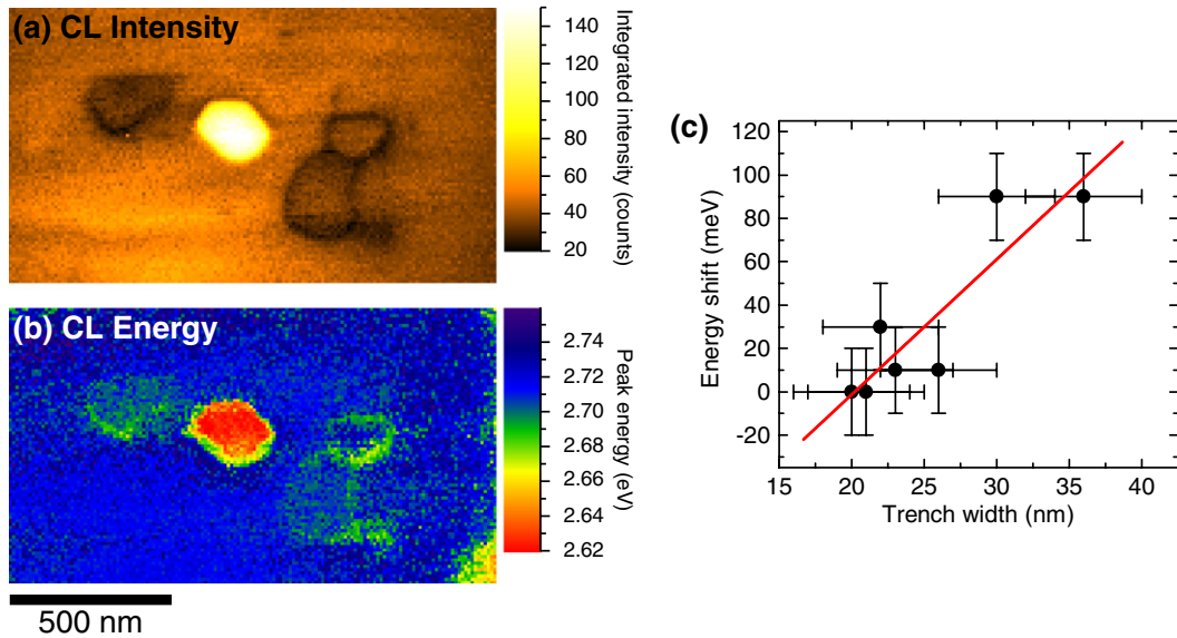
Figure 3. Room temperature CL maps gained by fitting the MQW emission peak in the hyperspectral data set with a Gaussian function: (a) integrated intensity and (b) peak energy map. (c) Energy shift of the inside region with respect to the surrounding area against trench width. The red line is a guide for the eye.
