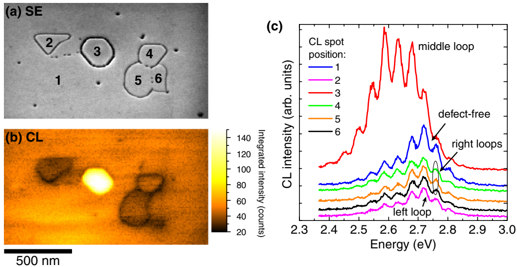
Figure 2. (a) SE image of three trench defects neighbouring each other, (b) panchromatic CL image of the same area as seen in the SE image and (c) CL spot spectra from six marked spots in the SE image. The spectra are offset for clarity.
