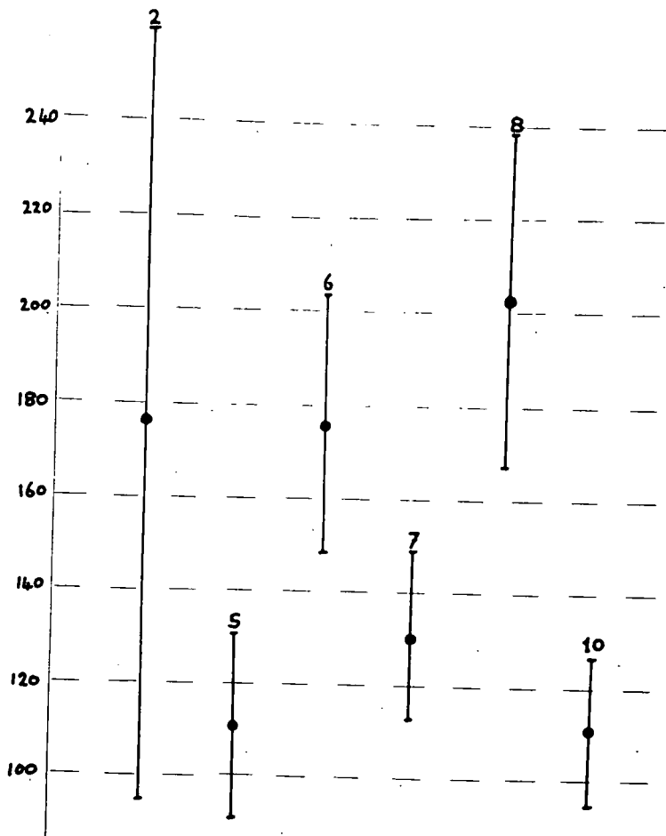
99.7% Confidence interval for a in equation iii.
