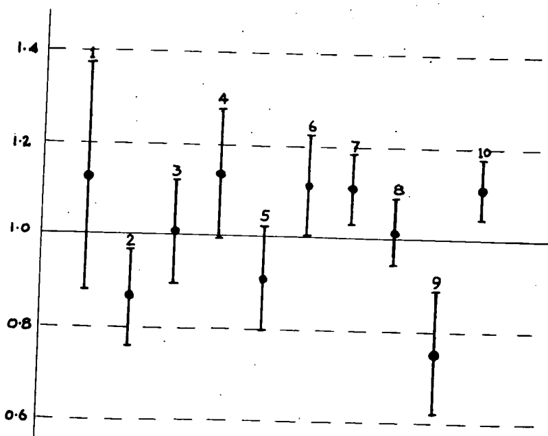
99.7% Confidence interval for power of F in equation ii.
