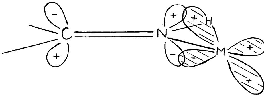
Fig.I.1(a) d\pi-\pi^* bonding involving a neutral methyleneamino-ligand
