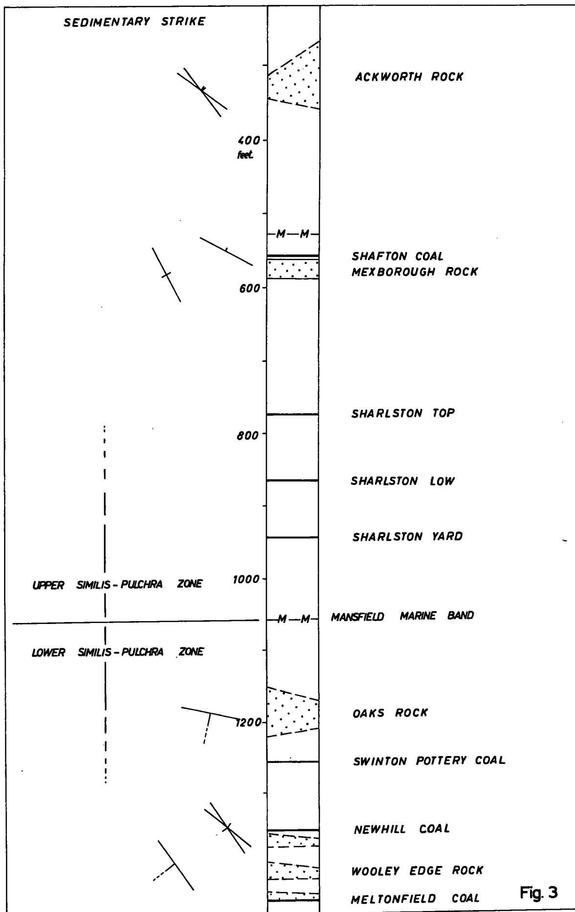
A GENERALISED STRATIGRAPHIC SECTION FOR THE REGION
