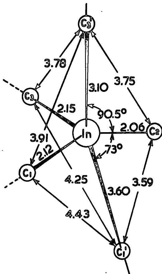
Trimethylindium. The arrangement of carbon atoms about indium
