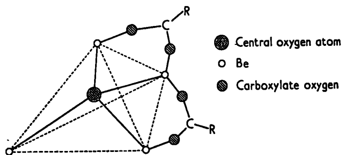
The structure of the carboxylate complexes \text{Be}_4\text{O}(\text{OOCR})_6 . Only two \text{RCOO} groups are shown.
