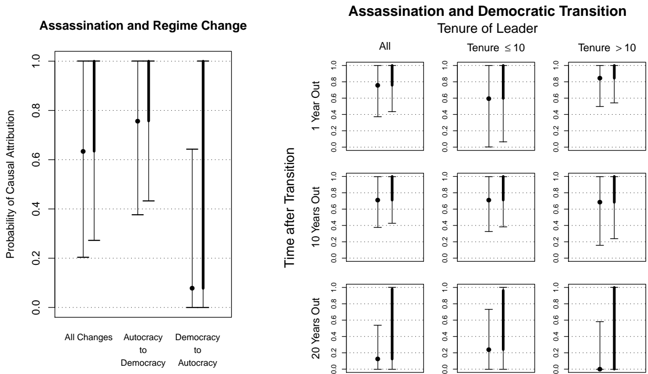
Figure 1: Assassination of Political Leaders and Regime Change. The pair of vertical lines in each plot represents the identification regions for the probability of causal attribution ( p_A ) under Assumptions 1 and 2 (solid circle on the left) and under Assumption 1 alone (thick bar on the right) along with their 95% confidence intervals (thin solid lines). The left panel shows the estimated probabilities that the regime changes observed after the assassinations of political leaders would not have happened had the assassination attempts failed. The right panel breaks down the estimated p_A for successful assassination and democratic transition by the tenure of the assassinated leader and by the time since the assassination. For a full description of the coding scheme for these groupings see Jones and Olken (2009). The results suggest that more than 75% of these democratic transitions can be causally attributed to the assassinations. The proportion is particularly large for the short-run moves to democracy following the assassination of long-tenured autocrats.
