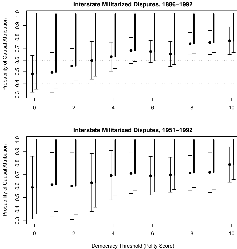
Figure 2: Proportion of the Past MID Onsets Attributable to the Lack of Democracy. In each panel, the horizontal axis represents the values of the Polity score used as the threshold for a dyad to be coded as democratic. The results in the top panel are based on the full dataset while the bottom panel is restricted to the post-war period. For the meaning of the graph components see the caption of Figure 1. The results suggest that the probability of causal attribution is roughly monotonically increasing as a function of the threshold for both time periods.
