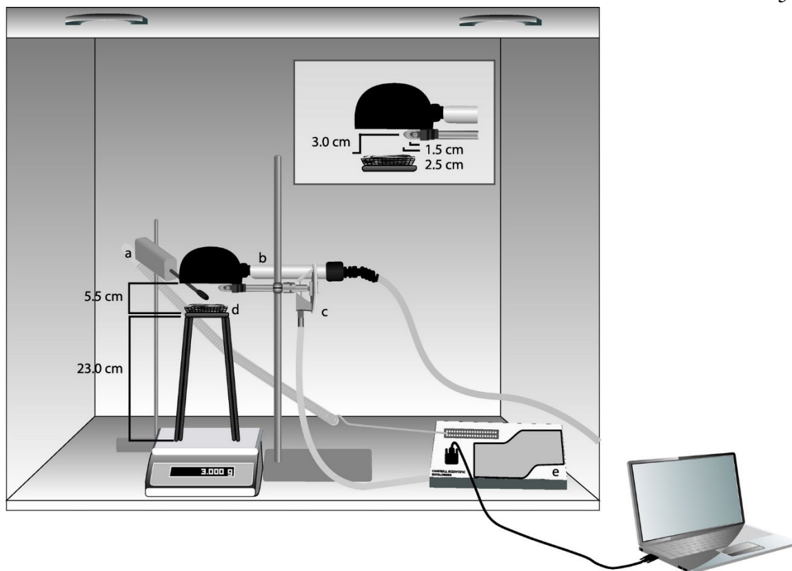
Fig. 3.1. Experimental setup for laboratory flammability testing: (a) type K thermocouple probe; (b) 500 W silica epiradiator; (c) pilot ignition source; (d) sample holder; and (e) data logger connected to scale and thermocouple.
