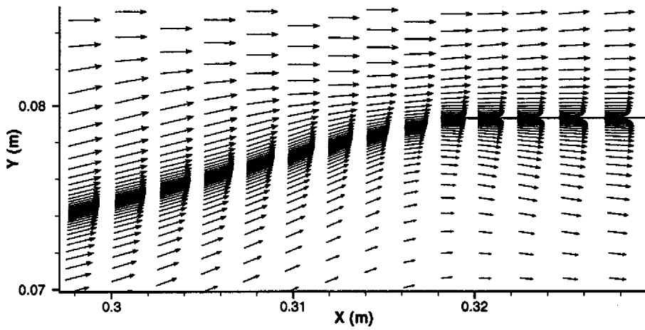
Figure 4: Velocity vectors near leading edge of splitter plate.
