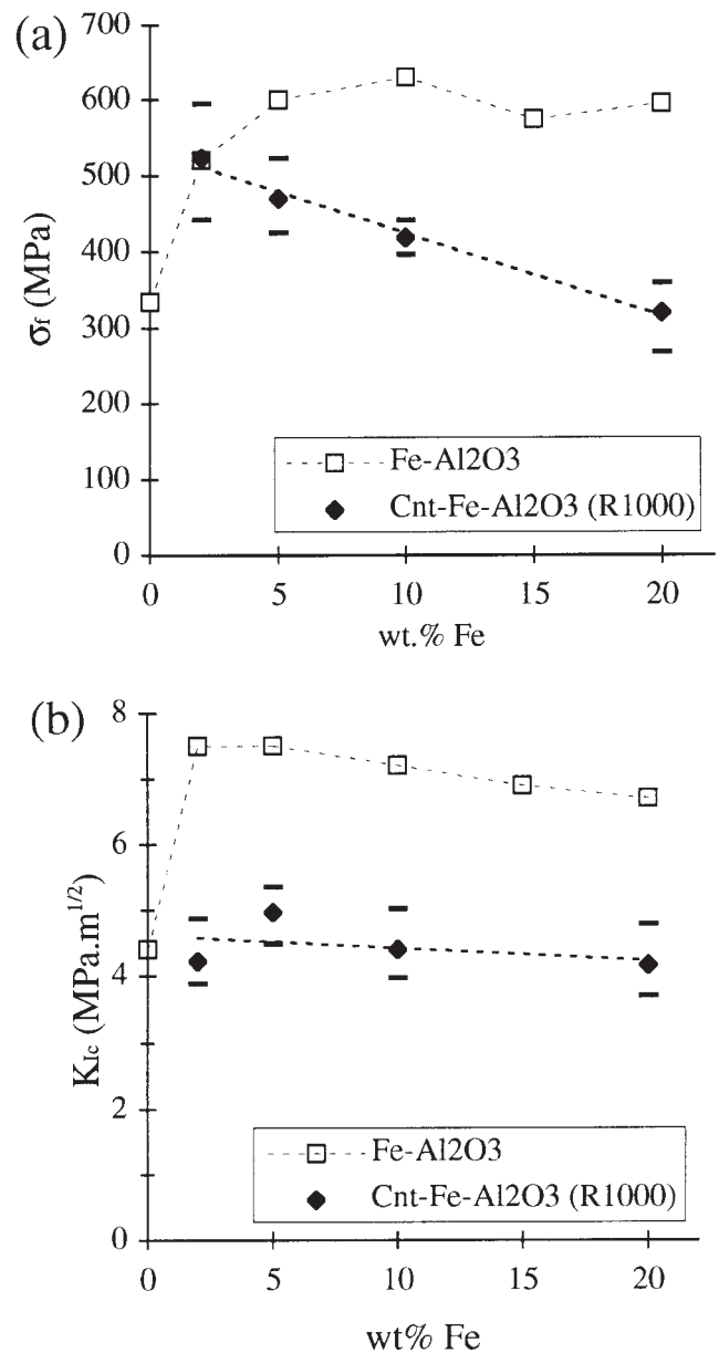
Fig. 5. (a) Fracture strength and (b) and fracture toughness of the dense composites prepared from powders reduced at 1000^\circ\text{C} (◆). The higher and lower measured values are also reported (≡). For the sake of comparison, the values obtained on carbon-free Fe– Al_2O_3 nanocomposites 14,15 are also shown (□). The dashed line is a guide to the eye.
