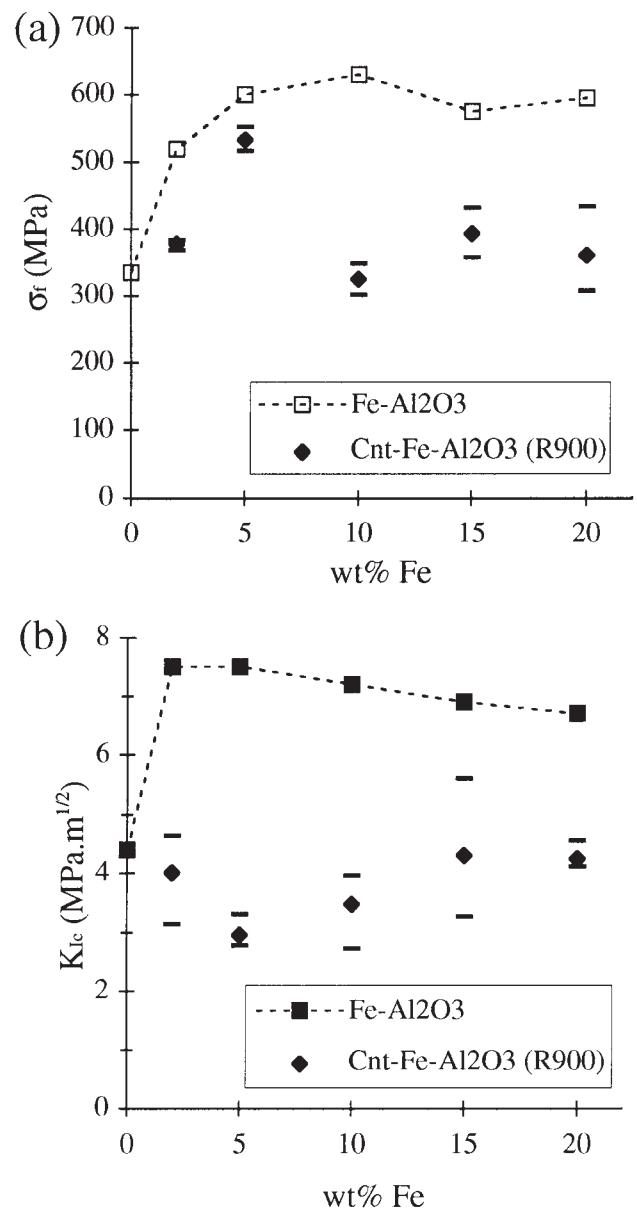
Fig. 4. (a) Fracture strength and (b) fracture toughness of the dense composites prepared from powders reduced at 900^\circ\text{C} ( \blacklozenge ). The higher and lower measured values are also reported ( \boxplus ). For the sake of comparison, the values obtained on carbon-free Fe- \text{Al}_2\text{O}_3 nanocomposites 14,15 are also shown ( \square ). The dashed line is a guide to the eye.
