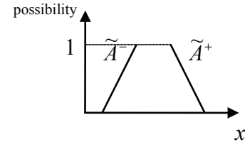
Fig. 3. Fuzzy number \tilde{A} = [\tilde{A}^-; \tilde{A}^+]
