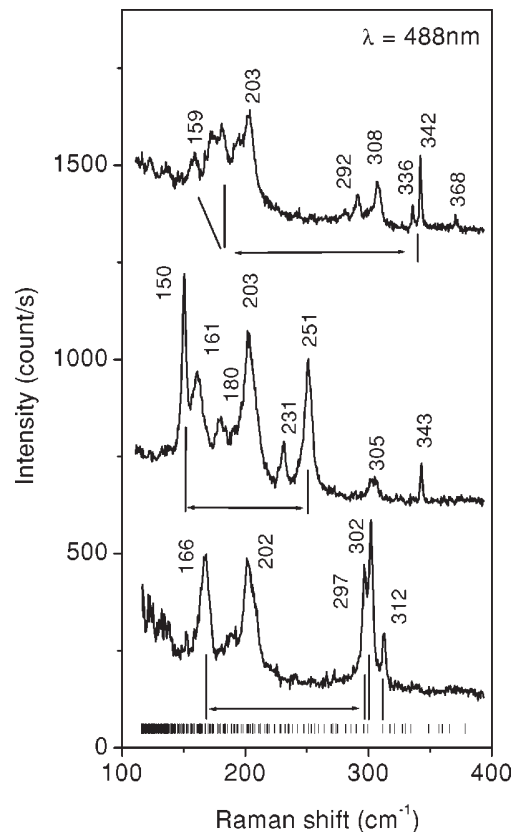
FIG. 2. Room-temperature Raman spectra of RB modes along a tube bundle containing double walled carbon nanotubes with different internal and external diameters.
