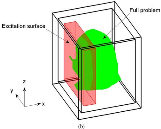
Fig. 1. DG-FDTD decomposition of a classical dosimetry problem. (a) First step: fine FDTD simulation. (b) Second step: coarse FDTD simulation.
