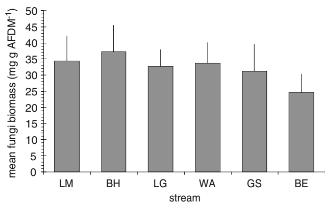
Figure 5 Mean ( \pm SD) fungi biomass in each stream. Streams are arranged following decreasing pH from the left to the right
