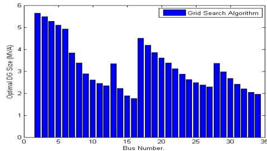
Figure 9. The optimal size of DG for each buses in 34-bus test RDS obtained by the classical grid search algorithm method.
