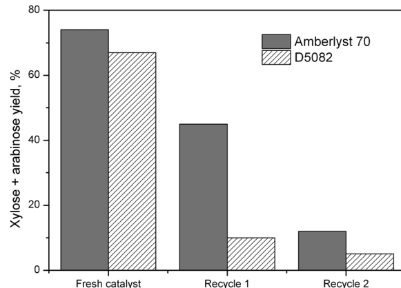
Fig. 4 Yield of xylose and arabinose after the recycling test using Amberlyst 70 and purolite D5082. Reaction conditions: xylan (0.1 g); catalyst (0.1 g); water (10 ml); 120\text{ }^\circ\text{C} , 10 bar Ar, 4 h.
