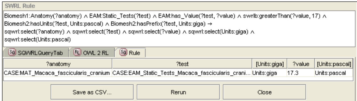
Figure 5: SQWRL query and results from the Biomech Ontology in Protégé
