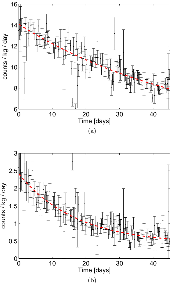
Figure 5: Activated Xe peak rates as a function of time, measured over part of the 85.3 day WIMP search run, beginning May 1, 2013. Peaks are measured for (a) ^{127}\text{Xe} , at 375 and 410 \text{keV}_{ee} , and (b) ^{131m}\text{Xe} , at 164 \text{keV}_{ee} . Best-fit exponential functions are shown with dashed lines (red, in color). The exponential slope of each function is fixed to the corresponding literature half-life listed in Table 4, and is not varied with the fit. Error bars are statistical.
