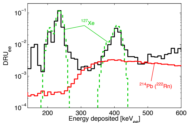
Figure 7: Constraint on ^{214}\text{Pb} in a 30 kg fiducial volume. Spectra are shown for measured data (black), simulation of ^{127}\text{Xe} peaks (gray dashed, green in color), and simulation of ^{214}\text{Pb} (gray solid, red in color). The ^{214}\text{Pb} activity shown is 32 \mu\text{Bq kg}^{-1} , measured to be the 90% upper limit from data in the range 300–350 keV ee .
