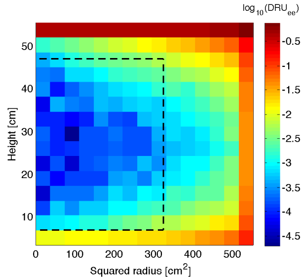
Figure 3: LUX \gamma ray ER background density in the range 0.9–5.3 \text{keV}_{ee} as a function of position, extrapolated from high-energy measurements based on Monte Carlo spectra. Rates are in units of \log_{10}(\text{DRU}_{ee}) . The 118 kg fiducial volume used in the 85.3 day WIMP search run is overlaid as the black dashed contour.
