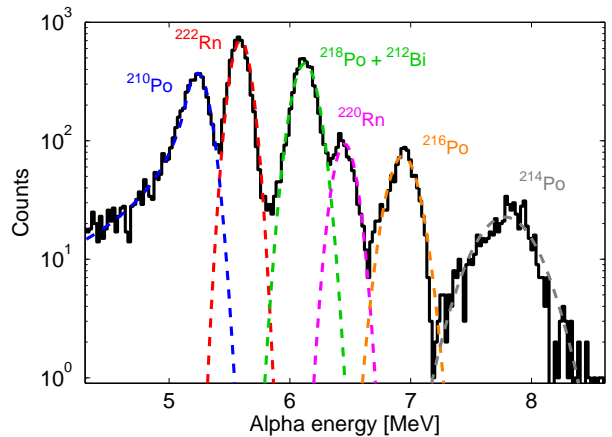
Figure 6: Signatures of \alpha particle decays in LUX WIMP search data in the active region. Energy is reconstructed from S1 measurements, calibrated on the observed location of the ^{222}\text{Rn} peak. Counts are collected over 6 livedays, spaced periodically over the course of the 85.3 day WIMP search run. Measured data (black) are fitted with Gaussian curves, with the exception of the ^{210}\text{Po} peak which is fit with a Crystal Ball distribution (see text for discussion). Fitted curves are shown in gray dashed (peaks shown in color online). Fitted curve peak values are fixed at the Q-values of the \alpha decays for all isotopes, with the exception of ^{210}\text{Po} where the peak value is the mean \alpha particle energy.
