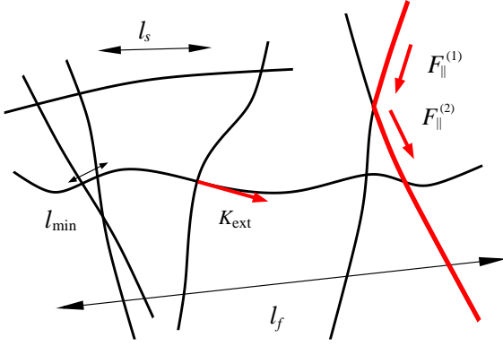
Fig. 1. Illustration of the local network structure and the relevant length-scales in the random fiber network (drawn in the deformed configuration): the fiber length l_f , the typical segment length l_s and the shortest deformed segment of length l_{\min} . K_{\text{ext}} signifies the bending force that the crossing fiber exerts in the axial direction of the horizontal fiber. F_{\parallel}^{(1)} and F_{\parallel}^{(2)} correspond to axial forces that are directly transmitted from one fiber to a neighboring fiber at the crosslink. This mechanism forms the basis for the establishment of force-chains; see main text.
