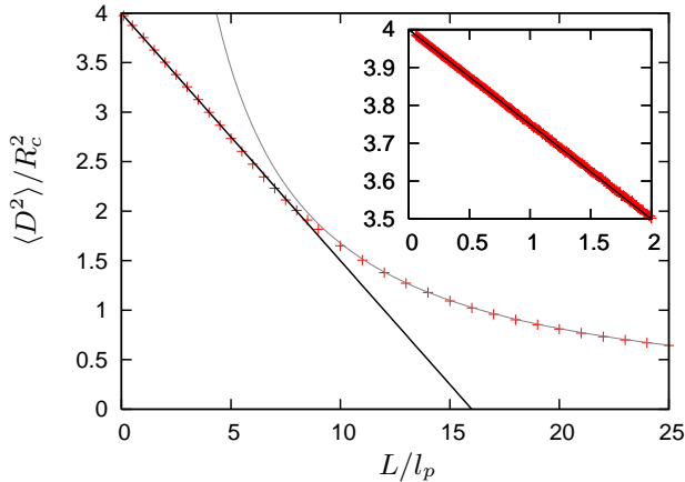
Fig. 3. Comparison of simulation data (crosses) for the mean square diameter \langle D^2 \rangle / R_c^2 versus L/l_p to equation (18) (black line). For L/l_p \gg 1 the mean square diameter decays with (L/l_p)^{-1} in accordance with previous results [16] (grey line). Error bars for the Monte Carlo data are approximately of the size of the symbols.
