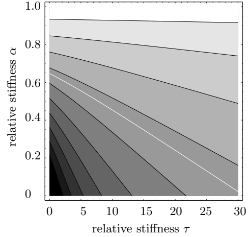
Fig. 2. Contour plot of the descent of the mean square diameter -\partial\langle D^2 \rangle / \partial(R_c^3/a_1) versus \alpha = a_1/a_2 and \tau = a_1/a_3 , where the contour lines decrease from \pi/2 at (\infty, 1) to 2/\pi at (0, 0) in ten equal steps. The additional white contour marks where in-plane and transversal fluctuations are equal in decreasing the diameter.
