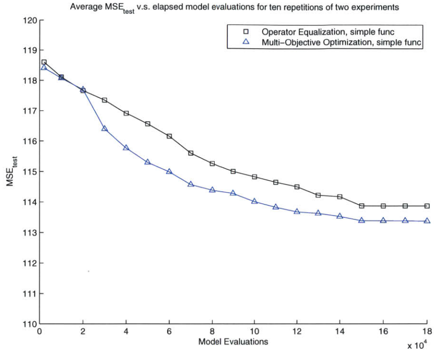
(a) \text{mean}(MSE_{test}) v.s. elapsed model evaluations for search-parallel experiments 1 and 2
