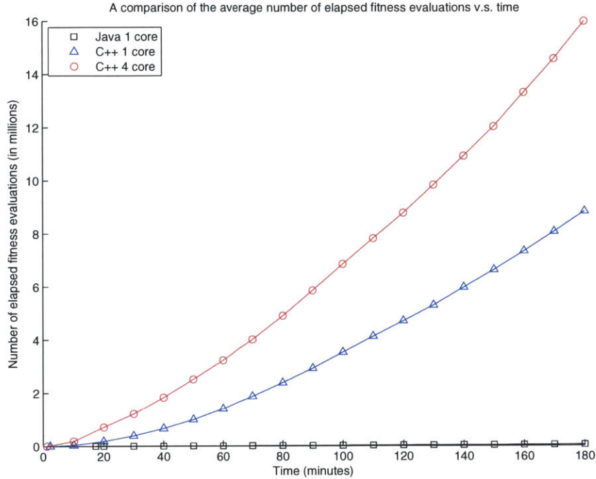
Figure 3-3: Average number of model evaluations made v.s. time for each of the 3 experiments
