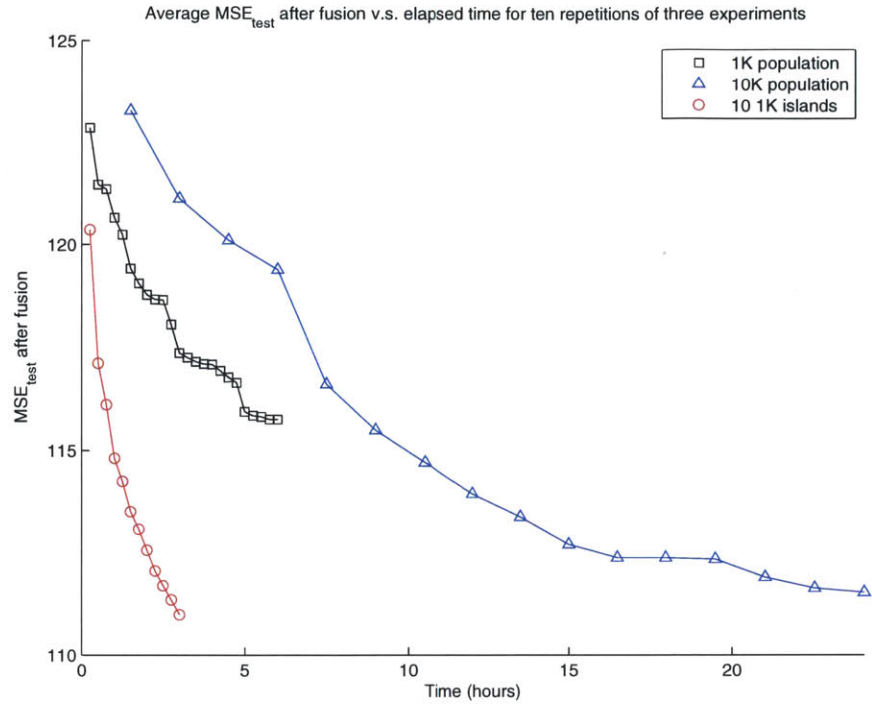
(a) MSE_{test} of population-parallel experiments
