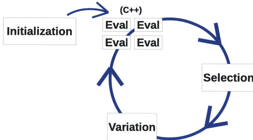
Figure 3-2: This figure visualizes FlexGP 2.0’s new evolutionary loop after the introduction of evaluation-level parallelism. Each labeled box represents a step in the loop. The four “Eval” boxes represent FlexGP 2.0’s parallelized C++ model evaluation . The blue path shows the flow of each population of models through the algorithm during each generation. In FlexGP the beginning of each generation occurs before the variation step.
