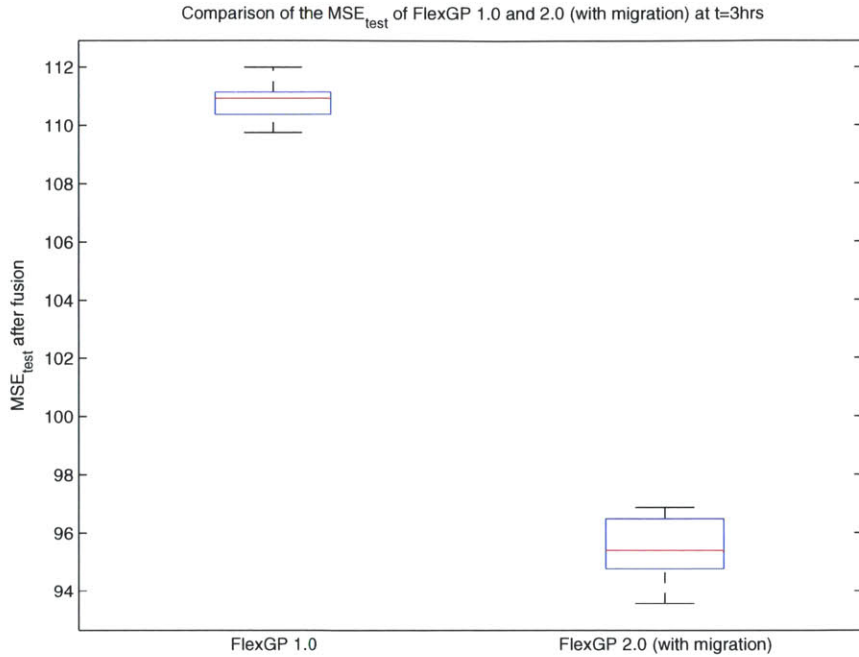
Figure 1-1: A comparison of the performance of FlexGP 2.0 v.s. FlexGP 1.0 after three hours of training. The boxplot represents the distribution of MSE_{test} values obtained after the fusion process. The specifics of the two experiments can be found in section 5.2.1.
