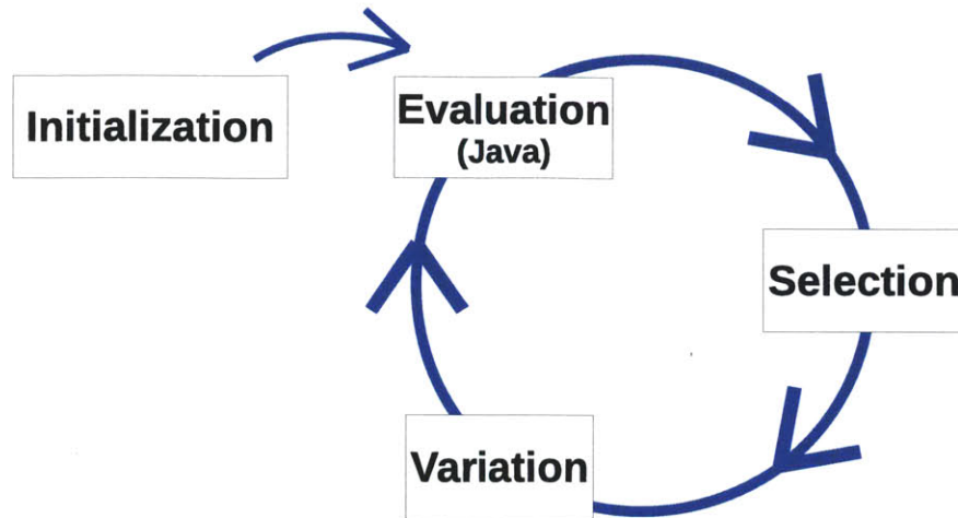
Figure 3-1: This figure visualizes the standard evolutionary loop used by FlexGP 1.0. Each labeled box represents a step in the loop. FlexGP 1.0 performs model evaluation in Java. The blue path shows the flow of each population of models through the algorithm during each generation. In FlexGP the beginning of each generation occurs before the variation step.
