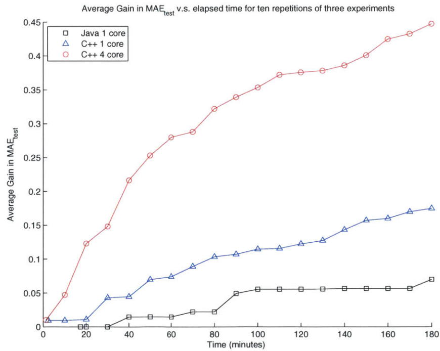
(b) Average gain in MAE_{test} v.s. time of evaluation-parallel experiments
