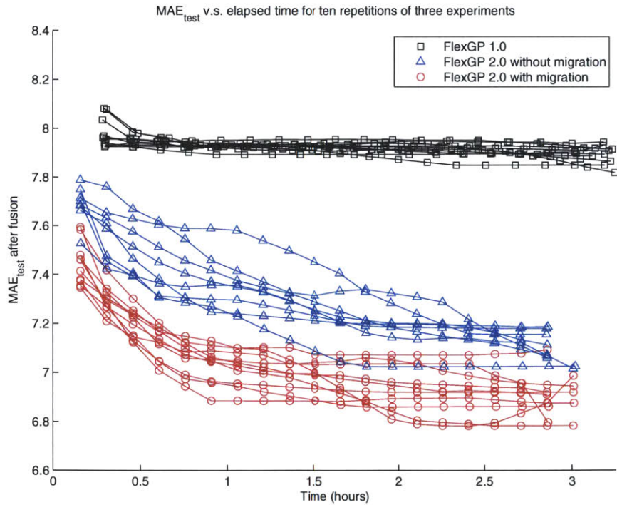
(b) MAE_{test} of total experiments
