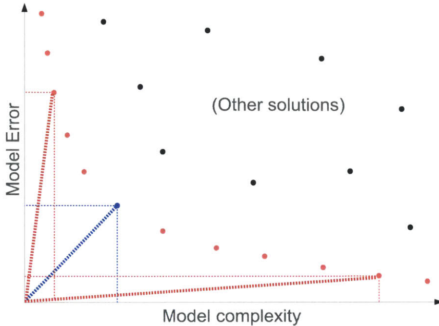
Figure 2-2: An example of using the euclidean distance to find the knee of a pareto front. The red dots represent models which are members of the pareto front, and the black dots represent other models under consideration. The two objectives under minimization are shown on the two axes. The euclidean distance of several models is shown by the diagonal dotted lines, where the blue dot shows the model with the lowest euclidean distance (the “knee”).
