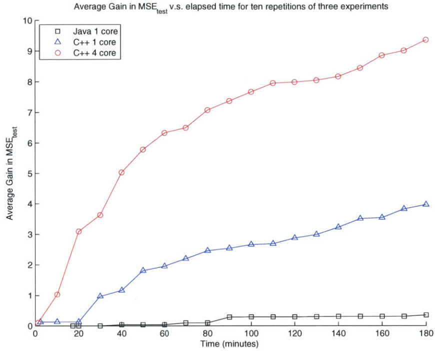
(a) Average gain in MSE_{test} v.s. time of evaluation-parallel experiments
