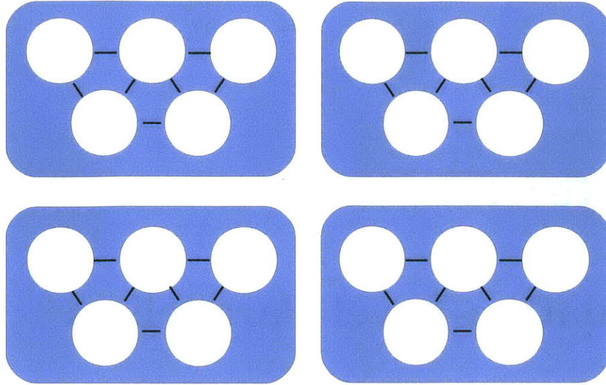
Figure 4-1: This figure depicts the combination of factor-level parallelism from FlexGP 1.0 with the population-level parallelism described in this chapter. Each blue box represents a unique factorization group with its own training and validation data split. Each white circle shows an independent population-parallelized node which sustains its own GP process. The lines between the population-parallelized nodes indicate a randomized topology for the communication of best models within each factorization group.
