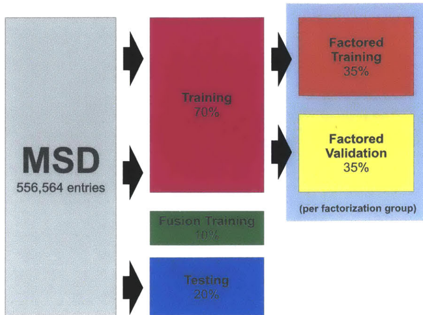
Figure A-1: A colorful depiction of the data partitioning hierarchy used in FlexGP. The original MSD is shown at left. The center column shows the training, fusion training and test datasets. The red and yellow boxes represent the factored training and validation data. If the user specifies a data factorization percentage, FlexGP will train on the factored training data in red. Otherwise, FlexGP will train on the magenta training data. The light blue box on the right indicates factorization occurs for each factorization group in FlexGP. The percentages shown are particular to the MSD problem, but the scheme is generalizable to other applications of FlexGP
