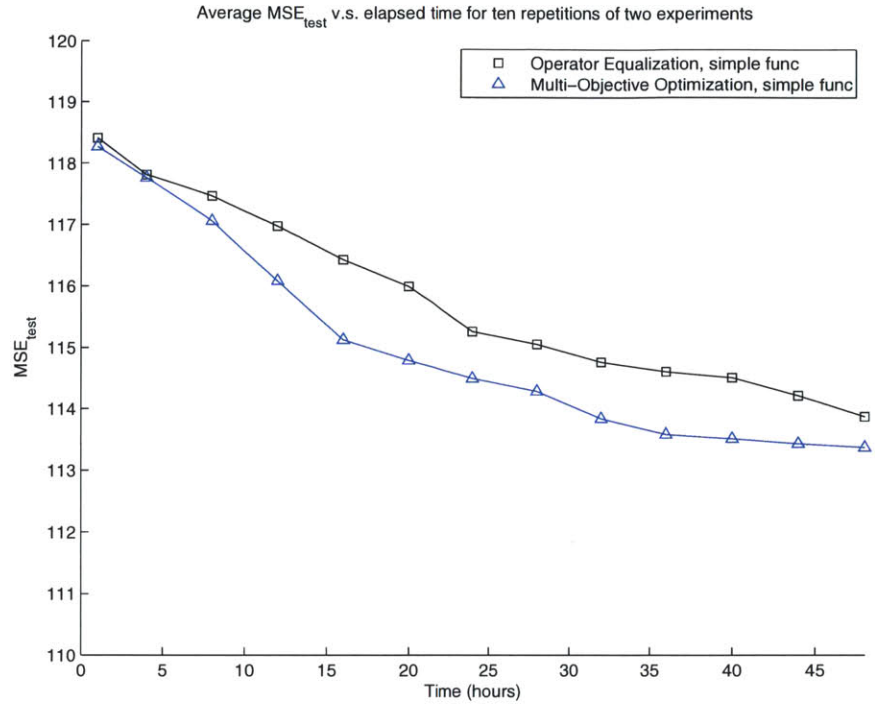
(a) \text{mean}(MSE_{test}) v.s. elapsed time for search-parallel experiments 1 and 2
