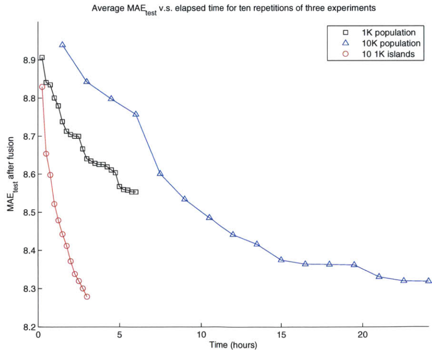
(b) MAE_{test} of population-parallel experiments
