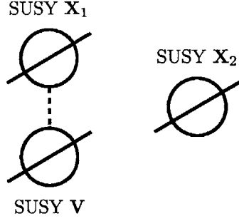
Figure 3-2: Decoupling of One Sector: When we decouple one sector from the visible sector, we simply have two distinct and unmixed sectors of supersymmetry breaking. The result is that sector 2, obtains a massless goldstino, and sector 1 together with the visible sector obtains a massless goldstino and a massive neutralino. Hence there is no state corresponding to the pseudo-goldstino.
