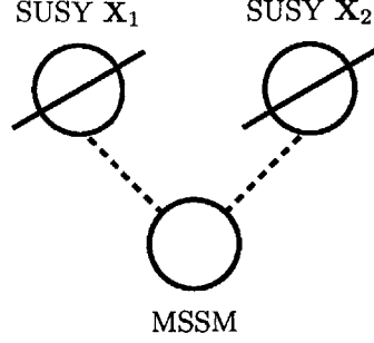
Figure 3-3: Breaking Scenario of MSSM: Unlike in the toy model, the visible sector of the MSSM does not break supersymmetry independent of the couplings to the hidden sectors.
