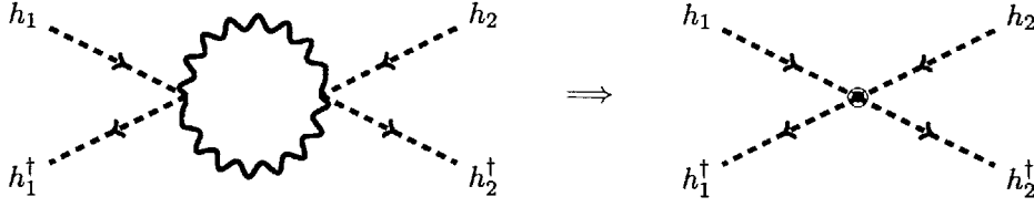
Figure 4-1: Perturbative Mass Generation in a Broken SU(N) Theory: Figure represents a term in the Coleman Weinberg expansion. When the intermediate gauge bosons are integrated out, we generate a mass term for the higgs fields.
