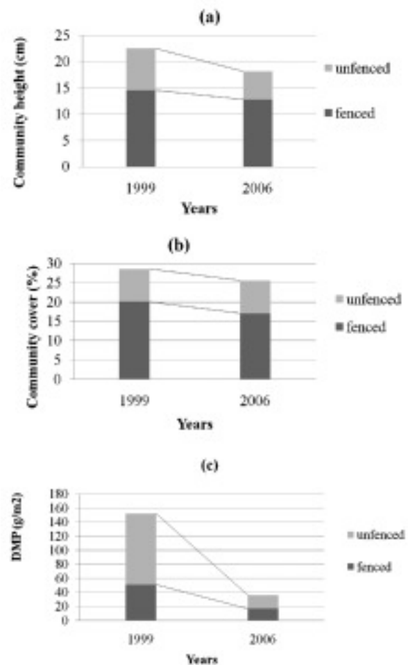
Fig. 2 Comparison of vegetation community of inside and outside of the fences (located in N43° 36'; E113° 55') (Were, (a) the community height (cm); (b) the community cover (%); and (c) Dry matter productivity (DMP) (g/m 2 ))
