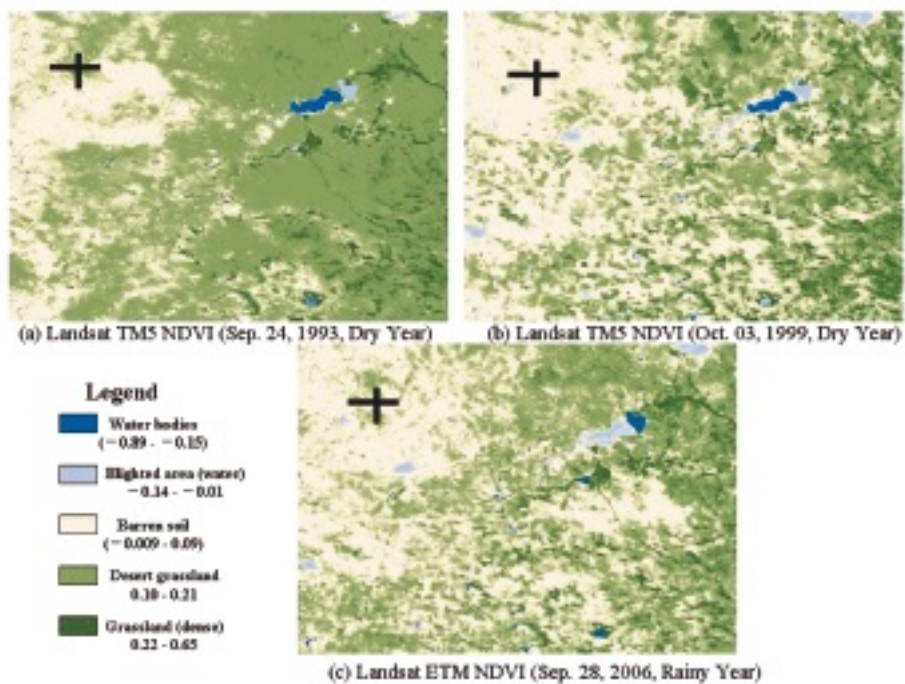
Fig. 5 Comparison of land degradation of grassland, with inside and outside of the fences in (a) Dry year: Sep. 24, 1993; (b) Very dry year: Oct. 03, 1999; and (c) rainy year: Sep. 28, 2006)
