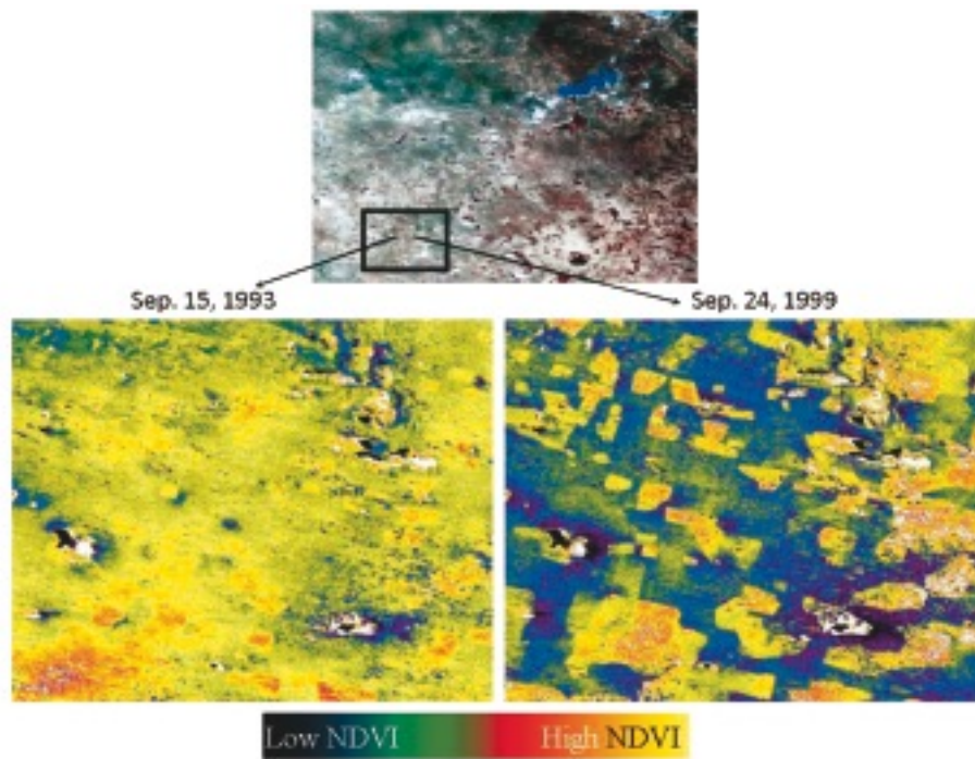
Fig. 4 Land cover change detection of fenced and unfenced area between 1993a and 1999a located in N42^{\circ} 21' - N43^{\circ} 07' ; E114^{\circ} 24' - E115^{\circ} 31'
