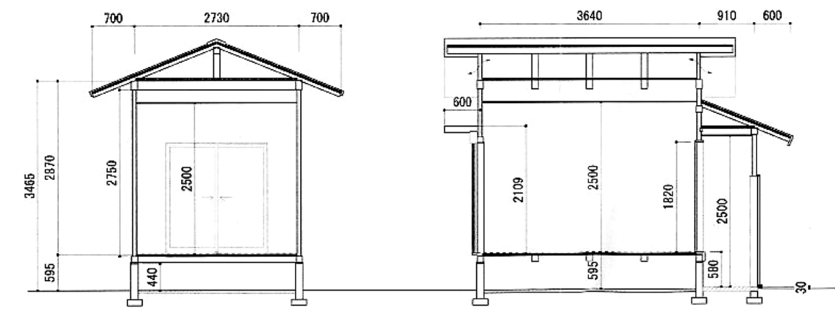
Figure 3. Scale of a test house: Model A
