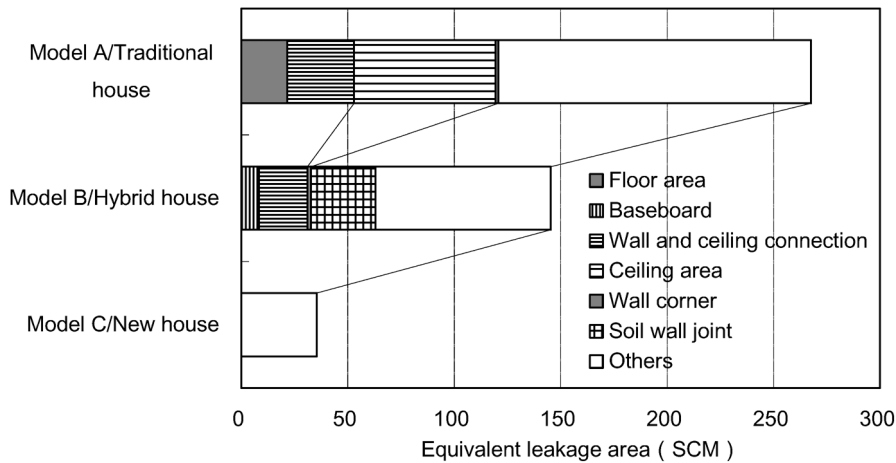
Figure 8. Measured equivalent leakage areas with sealing
