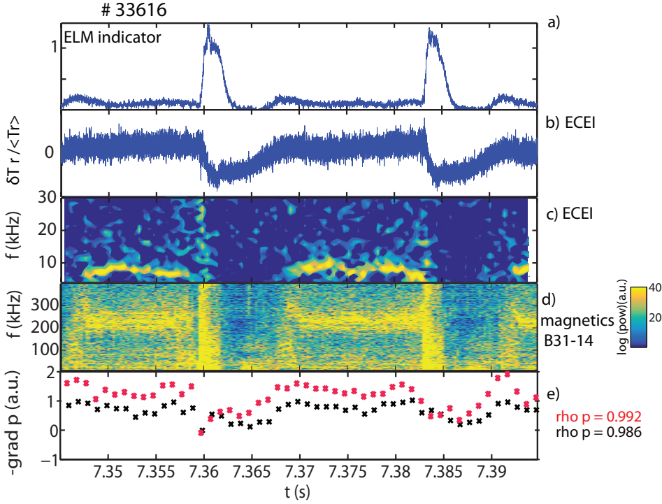
Figure 6: Shot # 33616. Temporal evolution of the: a) Divertor current. b) Relative change of the radiation temperature ( \delta T_r / \langle T_r \rangle ) measured by the single ECEI channel in the steep gradient region. Power spectral density comparison between: c) ECEI channel; d) magnetic pick-up coil; e) pressure gradient at two nearby radial locations in the steep gradient region. The position of both ECEI channel and the magnetic coil are indicated in figure 1.
