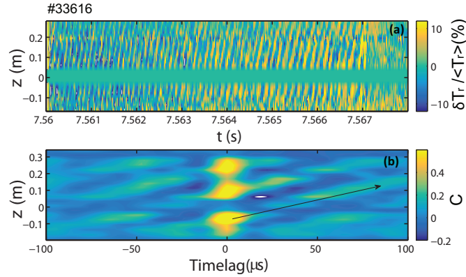
Figure 8: a) Vertically resolved \delta T_r / \langle T_r \rangle along the flux surface during the 8 kHz mode duration. b) Cross-correlation of the reference channel taken at the vertical position z = -0.1 m with all other poloidal channels. The black arrow approximates the direction of the mode propagation in space and time.
