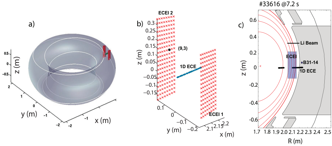
Figure 1: a) q = 6 flux surface plotted as a gray shaded area for the shot # 33616 at t 7.2 s. Magnetic field line for this equilibrium is plotted as white solid line. The red surfaces, intersecting the q = 6 flux tube correspond to two ECEI imaging systems. b) Absolute measurement positions of two toroidally separated ECEI arrays in Cartesian coordinates are shown as red crosses (X); edge channels of conventional ECE radiometer are shown as green dots. The ECEI channel of the ECEI 2 array that is used for comparison with the magnetic measurements is marked as black circle ( \bullet ). c) Poloidal cross section of ASDEX Upgrade indicating the measurement positions of: the Lithium beam diagnostic, ECE Imaging, standard ECE radiometer and magnetic pick-up coil (B31-14).
