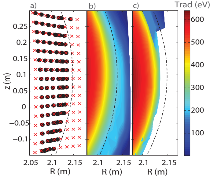
Figure 4: Shot # 33616 at 7.5 s. a) Calculated cold resonances are labelled as red crosses (X) and the warm resonances as black circles ( \bullet ). The radiation temperature mapped onto positions of the cold resonances (b) and the warm resonances (c). The separatrix position is marked by a black dashed line.
