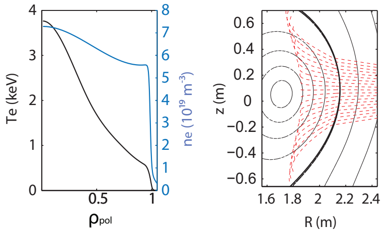
Figure 2: a) T_e and n_e profiles used to forward model the radiation transport. b) Ray tracing representing the lines of sight for 20 ECEI poloidally distributed channels.
