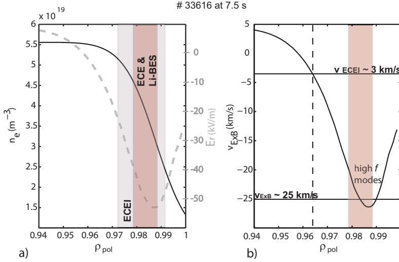
Figure 11: Shot # 33616 at t = 7.5 s. a) Density profile of the steep gradient edge region shown as a black solid line; radial electric field E_r estimated from the poloidal flow of impurities is presented as a dashed gray line. Radial resolution of the edge diagnostics used in this work is color coded: red corresponding to the Li-BES and 1D ECE channel; grey corresponding to the ECEI channel. b) E \times B velocity calculated using the E_r . The vertical dashed line shows the position of the mode in case the velocity of the mode would match exactly the E \times B velocity.
