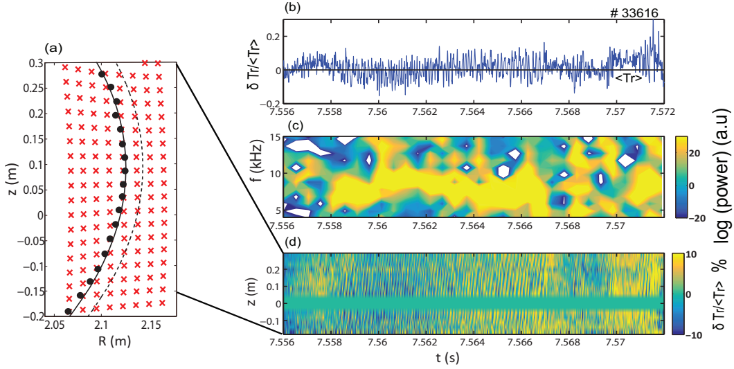
Figure 7: Localization and the temporal evolution of \delta T_r / \langle T_r \rangle seen in the ECEI observation window. a) Warm resonant channels ( \bullet ) of array 2, that measure the modulation of the radiation temperature, are distributed along the flux surface at \rho_{pol} \sim 0.985 . (b) Relative temperature change of a single channel 10 cm above the midplane. (c) Time resolved spectrogram of the channel as in (b) showing the presence of the strong mode in the 7 - 8 kHz range. (d) Temporal evolution of \delta T_r / \langle T_r \rangle in percentage measured by the channels distributed along the flux surface with positions shown in (a) as black bullets. This representation visualize the propagation of \delta T_r / \langle T_r \rangle in the poloidal direction, from the bottom to the top channels, along the flux surface. Three channel at the midplane ( z=0 ) are set to zero.
