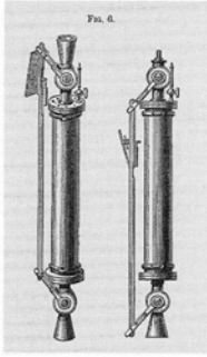
"Buchanan's" deep-sea water bottle. "ブキャナン作" 深海用採水器
