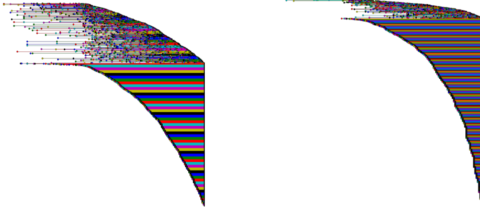
Figure 6: Barcodes of homological cycles in H_1 (left) and H_2 (right), ordered for their death time. The left and right endpoints of each segment represent the first and last step in the filtration where the hole appears.
