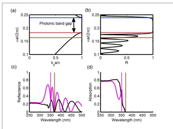
Fig. 1 (a) Photonic band diagram at normal incidence of infinite 1D photonic crystal ( d_1=40.5 nm, d_2=0.5 \times d_1 , n_1=2.8 , n_2=1.33 ). (b) Reflectance spectrum of red-edged tuned BR slab ( d_1=40.5 nm, d_2=0.5 \times d_1 , N=10 ) with \text{TiO}_2 extinction coefficient set artificially to zero. (c) Reflectance spectrum of the same slab as (b) but calculated with complex refractive index of anatase \text{TiO}_2 . (d) Absorption spectrum of the same slab as (c). In (a, b), horizontal red (blue) dashed lines indicate red (blue) edge of the photonic band gap; horizontal brown dashed line indicates \text{TiO}_2 electronic band edge. In (c, d), vertical magenta (brown) dashed lines indicate red edge wavelength ( \text{TiO}_2 electronic band edge wavelength). Normal incidence is assumed (incidence medium: water, substrate: glass). Reflectance and absorption spectra of the reference slab (black curves) are also shown (c, d).
