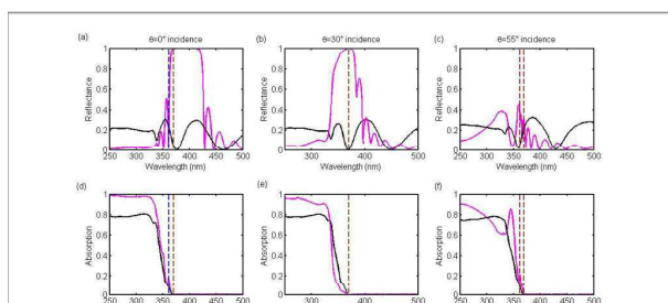
Fig. 9 Reflection (a, b, c) and absorption (d, e, f) of IO slab with D=167 nm and f=0.12 (open porosity). Vertical red (blue) dashed lines indicate positions of red (blue) edge of the photonic band gap. Non-polarized light, \phi=-30^\circ , \theta=0^\circ (a, d), \theta=30^\circ (b, e), \theta=55^\circ (c, f). For comparison, reflectance and absorption spectra of reference slabs are also shown.
