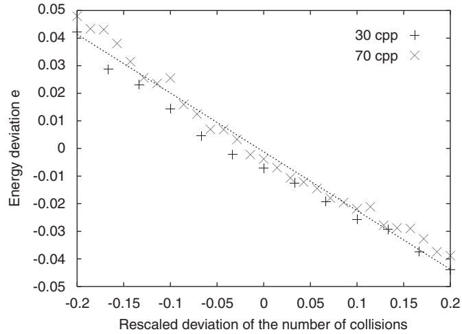
Fig. 2. Energy deviation e = \langle E \rangle_{\Delta} - 1 as a function of the rescaled deviation of the number of collisions \delta = \Delta/t , after 30 and 70 collisions per particles (cpp). The gas is composed of 10 000 000 particles with \alpha = 0.8 . The dashed line is the linear fit Eq. (6) of this relation.
