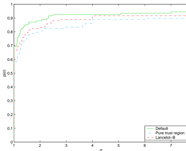
Figure 4.1: Iterations performance profiles for the two variants and LANCELOT B.
