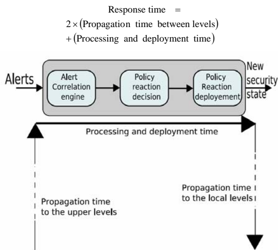
Figure 4. Response time.
