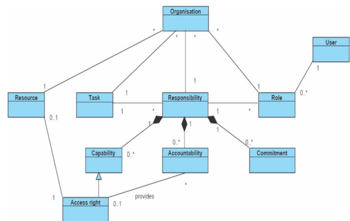
Figure 1. UML Model of Responsibility
