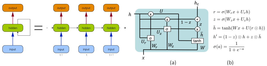
Figure 2: Structure of recurrent neural network.
