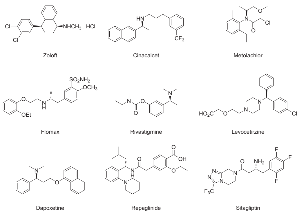
Figure 1. Selected pharmaceuticals and agrochemicals containing chiral amines.
