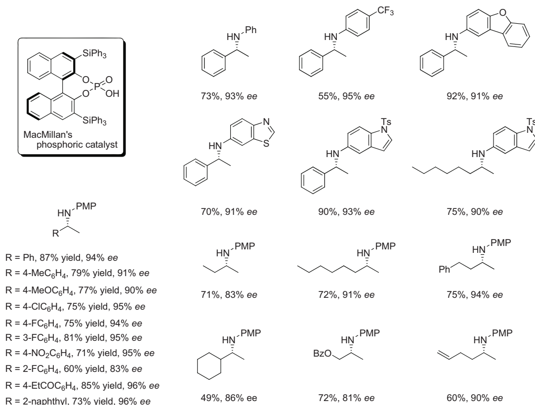
Scheme 19. Results of organocatalytic asymmetric reductive amination of ketones by MacMillan.
