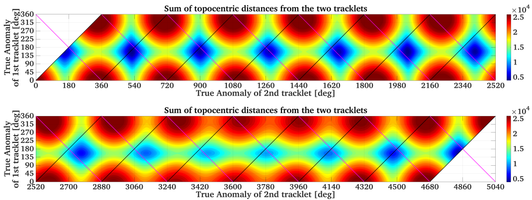
(c) Sum of the Object-Observer Distance for the 1st and 2nd tracklet
