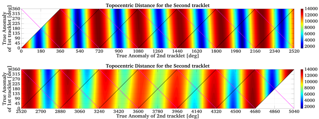
(b) Object-Observer Distance for the 2nd tracklet
