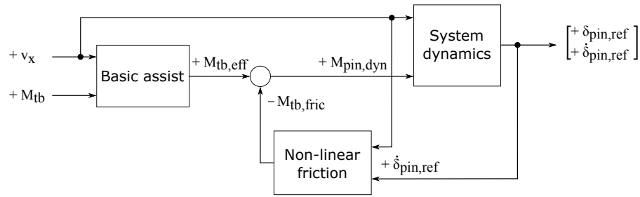
(a) Reference generator for admittance control
