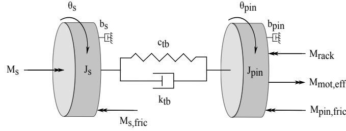
Figure 2.2: Free body diagram of a simplified electric power assisted steering system with 2-DOF (degree of freedom); steering angle and pinion angle (or equivalent to rack displacement).
