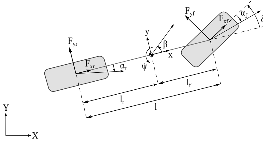
Figure 2.6: Single track vehicle model in global coordinate system.
