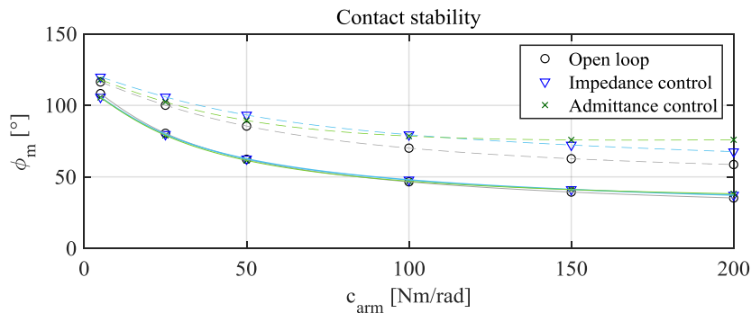
Figure 3.11: SbW-FFb driving port admittance loop gain phase margin as a function of drivers' arm stiffness. The figure shows \phi_m variation for open loop, impedance and admittance control for J_{arm} = 0 \text{ kgm}^2 (---) and J_{arm} = 0.07 \text{ kgm}^2 (—) respectively.
