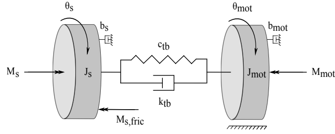
Figure 2.5: Free body diagram of a steer-by-wire force-feedback system with 2-DOF; steering angle and motor angle.
