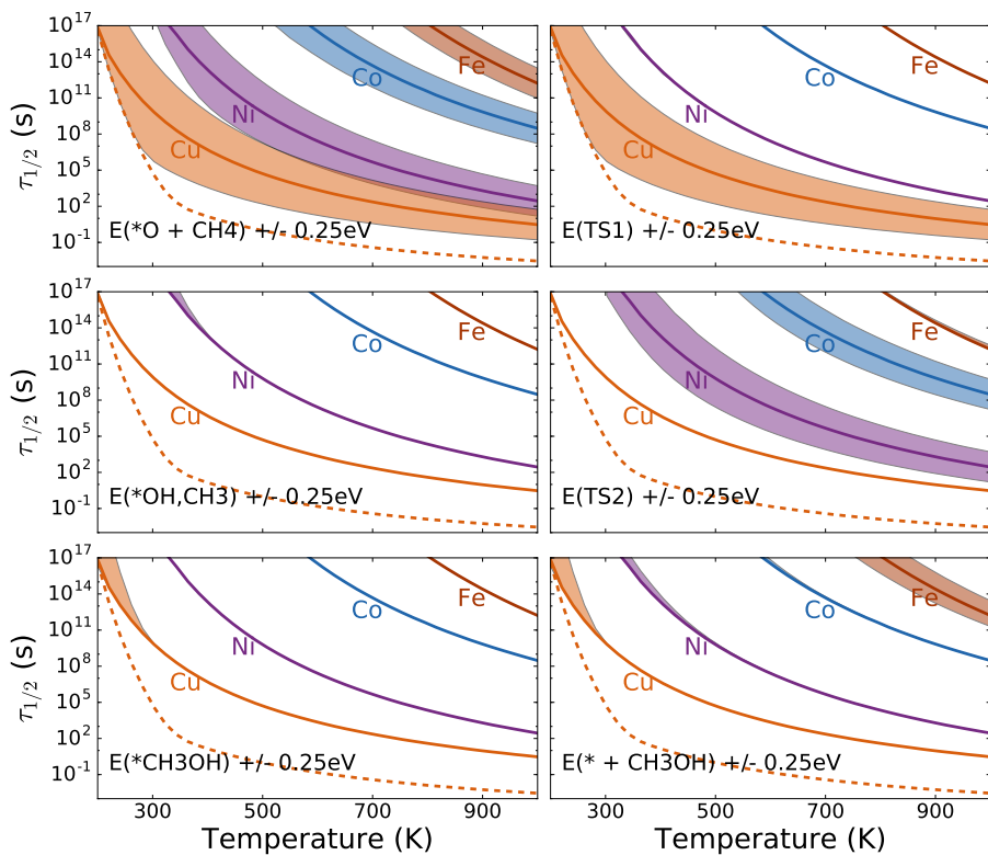
Figure 4.8: Change in \tau_{1/2} when changing the energy of each intermediate by \pm 0.25 eV. From Paper I .
