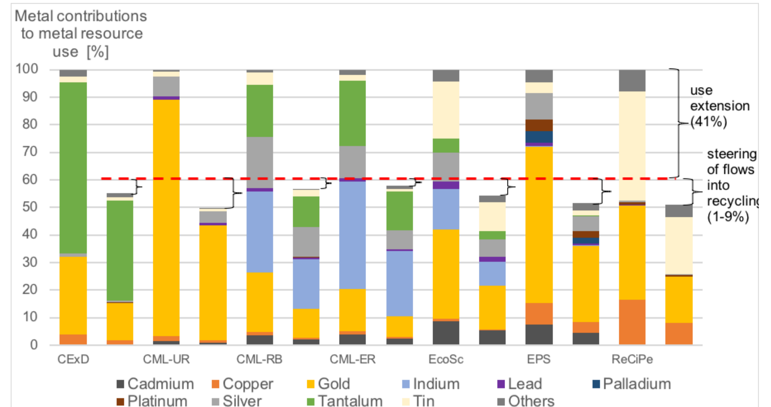
Figure 2. Metal resource use impacts: the reuse alternative compared to the new laptop alternative [%] with five impact assessment methods of which one has three versions. Metals with >1.5% contribution with at least two methods or >4% with at least one method are displayed individually. Others include 20 metals such as aluminium, iron, nickel and rare earth elements.
