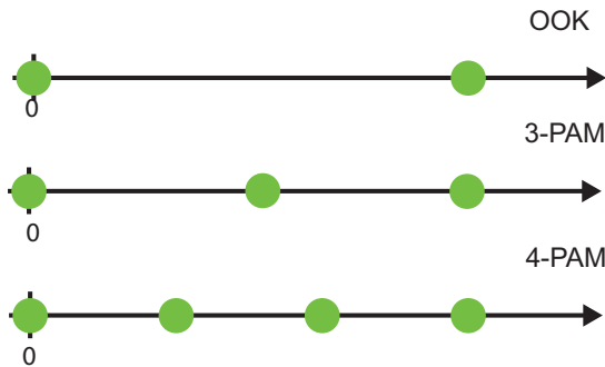
Figure 3.1: Constellation diagrams for OOK and 4-PAM
