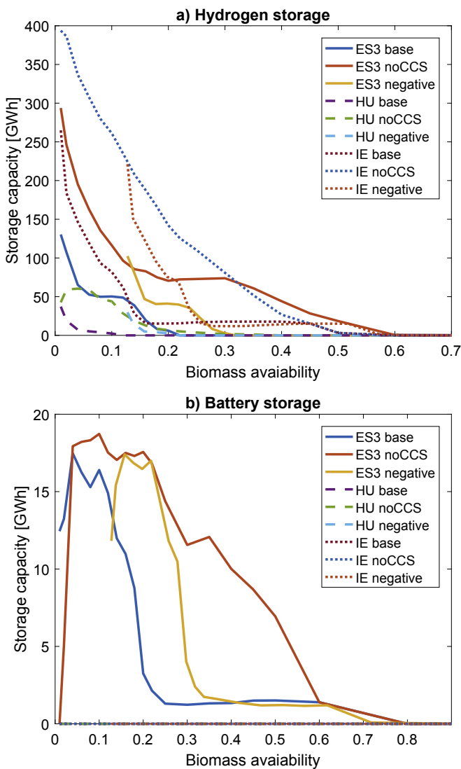
Fig.4. Storage capacities of; (a) hydrogen; and (b) batteries.
