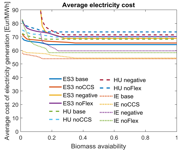
Fig.6. Average electricity generation cost for each case and region. The biomass cost is included by multiplying the marginal value of biomass to the biomass usage until the marginal biomass value reaches 30 €/MWh th after which the cost is set constant.
