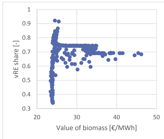
Fig. B.2. The vRE share is plotted against the biomass value for the base case in ES3 with 20% biomass availability.
