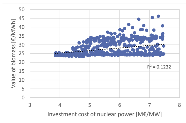
Fig. B.1. The value of biomass as function of the investment cost of nuclear power plants.
