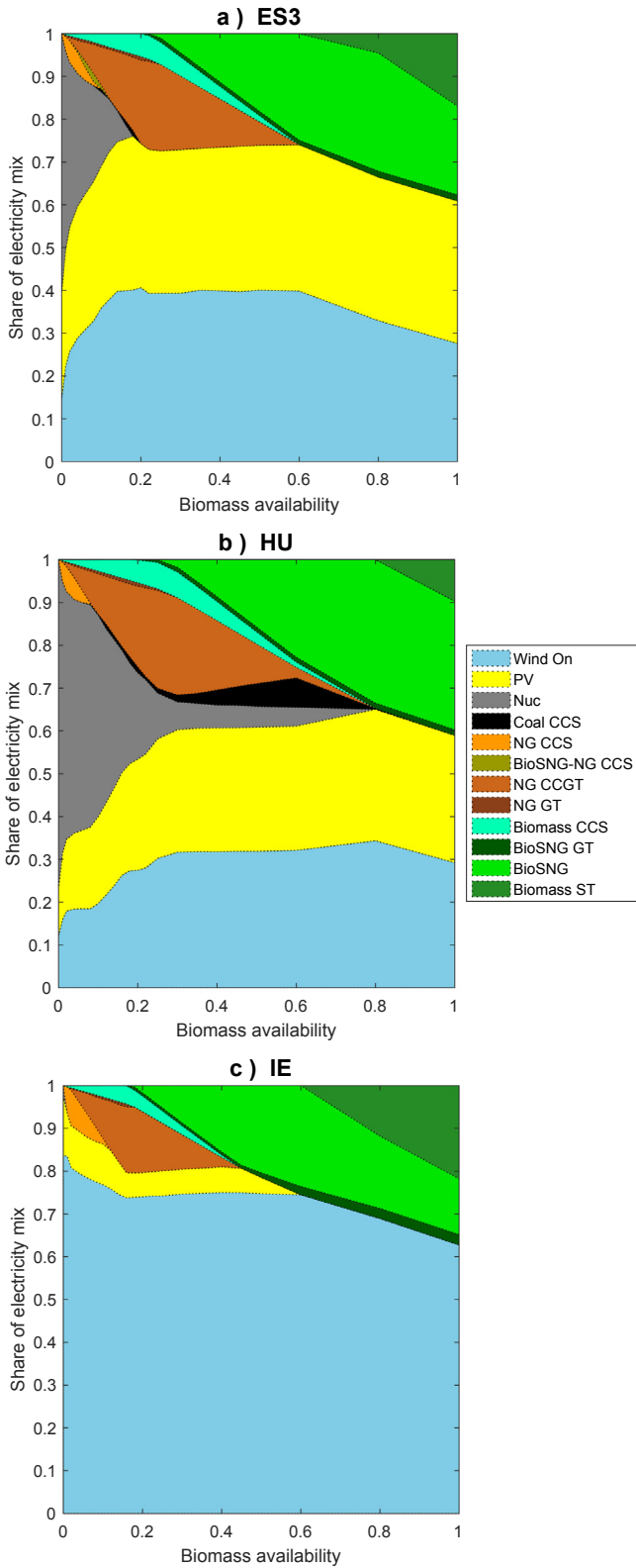
Fig. 1. The electricity mixes for different levels of biomass availability for the three regions in the base case.
