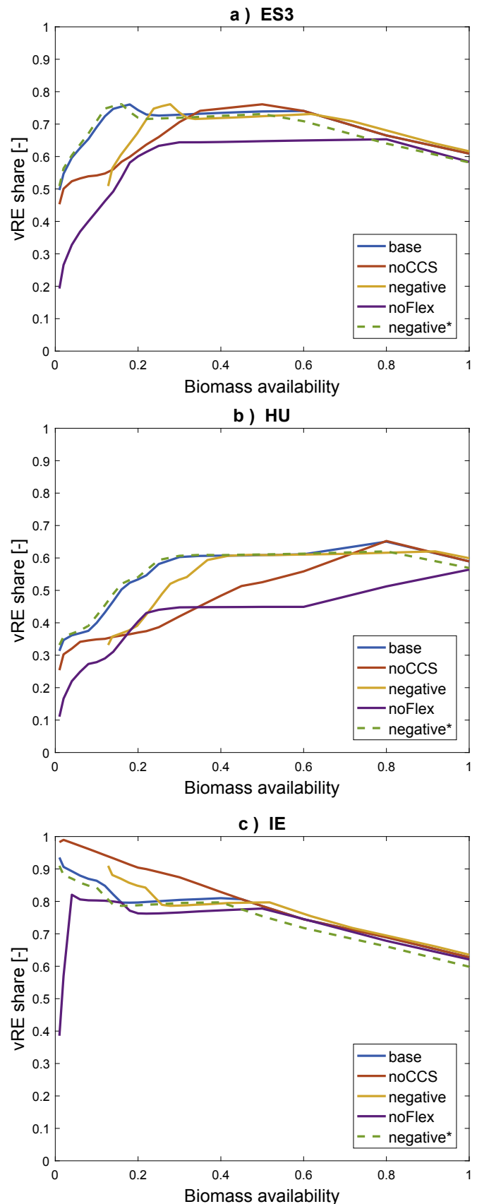
Fig. 3. The vRE share as function of the biomass availability levels. The green line represents the scenario “negative*”, where the biomass needed for negative emissions is excluded from the availability, i.e., the curve is shifted.
