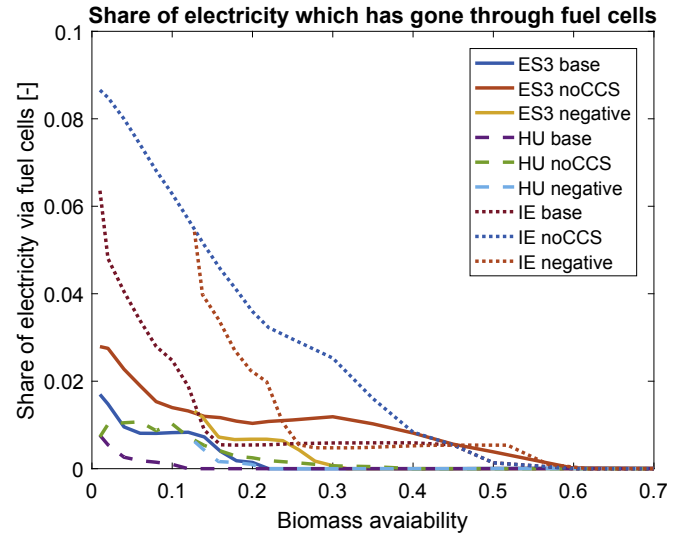
Fig.5. Share of electricity that is (re)generated in fuel cells.
