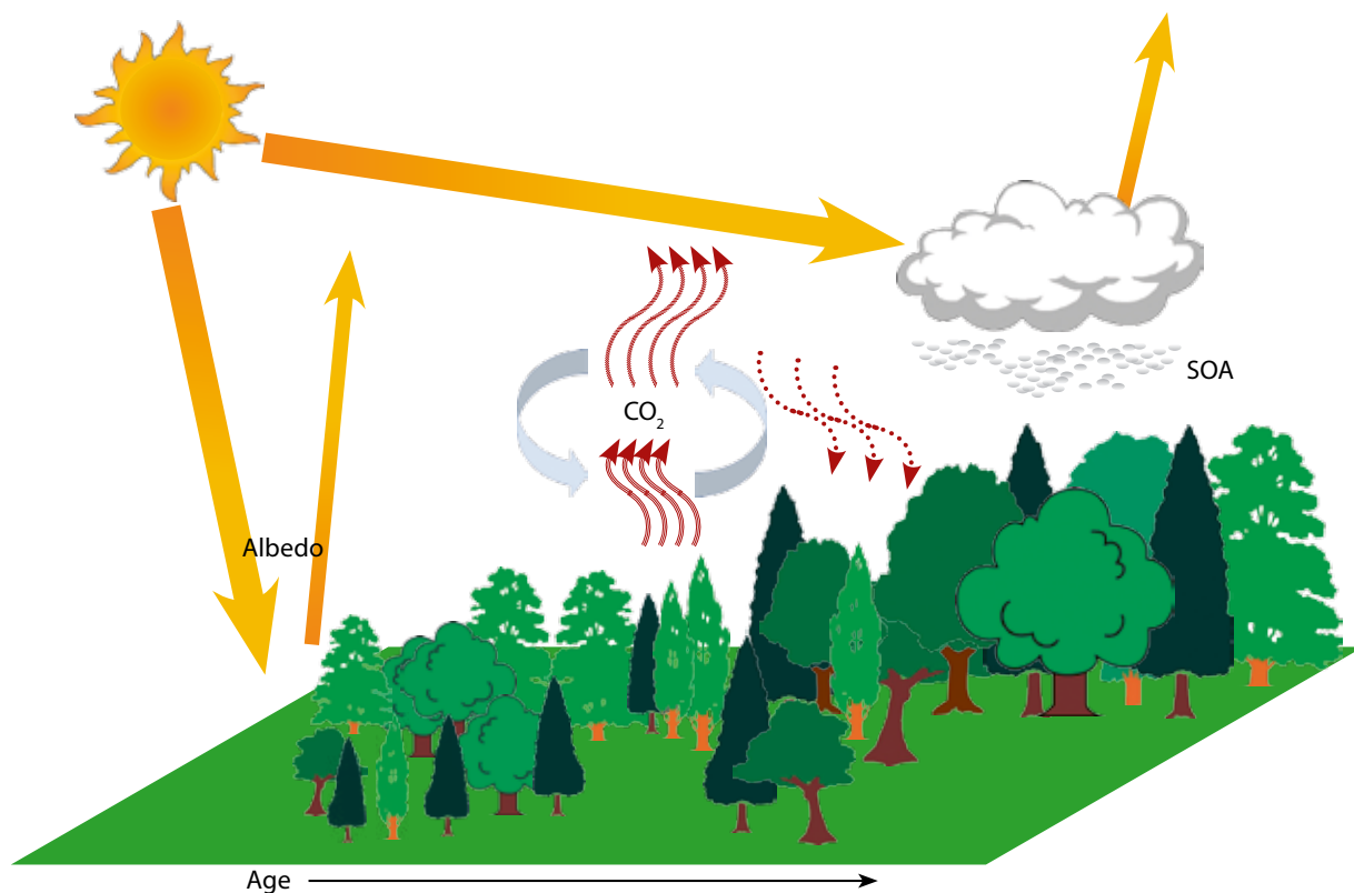
Figure 8. The main processes that influence radiative forcing: surface albedo, CO 2 , and secondary organic aerosols, SOA. The yellow arrows indicate direct radiation from the sun, and the red arrows represent infrared radiation.
