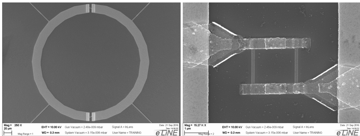
Figure 1. SEM view of single annular ring antenna (left panel) with two identical SINIS bolometers (right panel).
