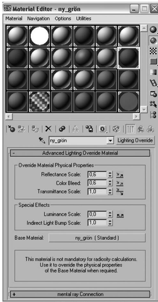
Figure 4.7. The parameters in 3Ds max® describing colour bleeding and reflectance.
