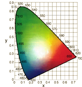
Figure 2.7. CIE's chromaticity diagram. (Image courtesy of Nave, C.R., 2009: http://hyperphysics.phy-astr.gsu.edu/hbase/HFrame.html )
