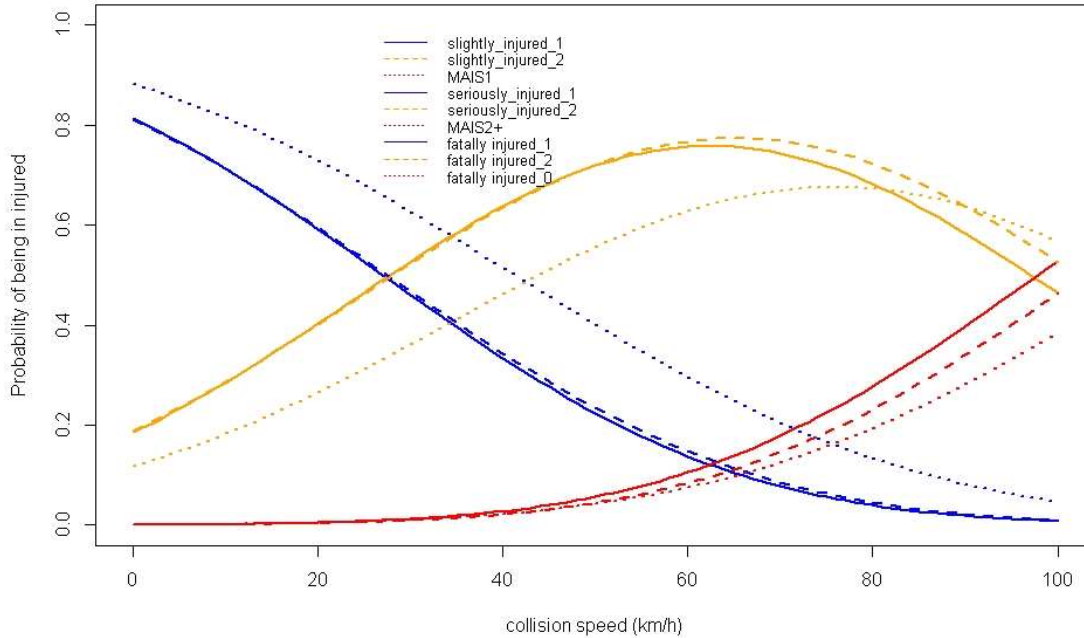
Figure 103: All IRF for pedestrians plotted together.
