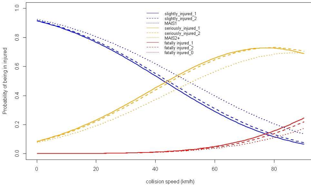
Figure 101: IRF for cyclists based both on police coding and MAIS.
