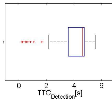
Figure 56: Box plot of detection times for UC_DEM_11 without view obstruction.
