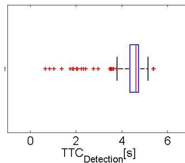
Figure 26: Box plot of detection times for UC_DEM_4 without view obstruction.
