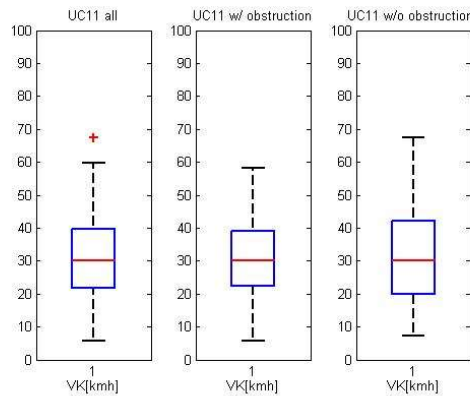
Figure 58: Box plots of the collision speed of the vehicle in UC_DEM_11.
