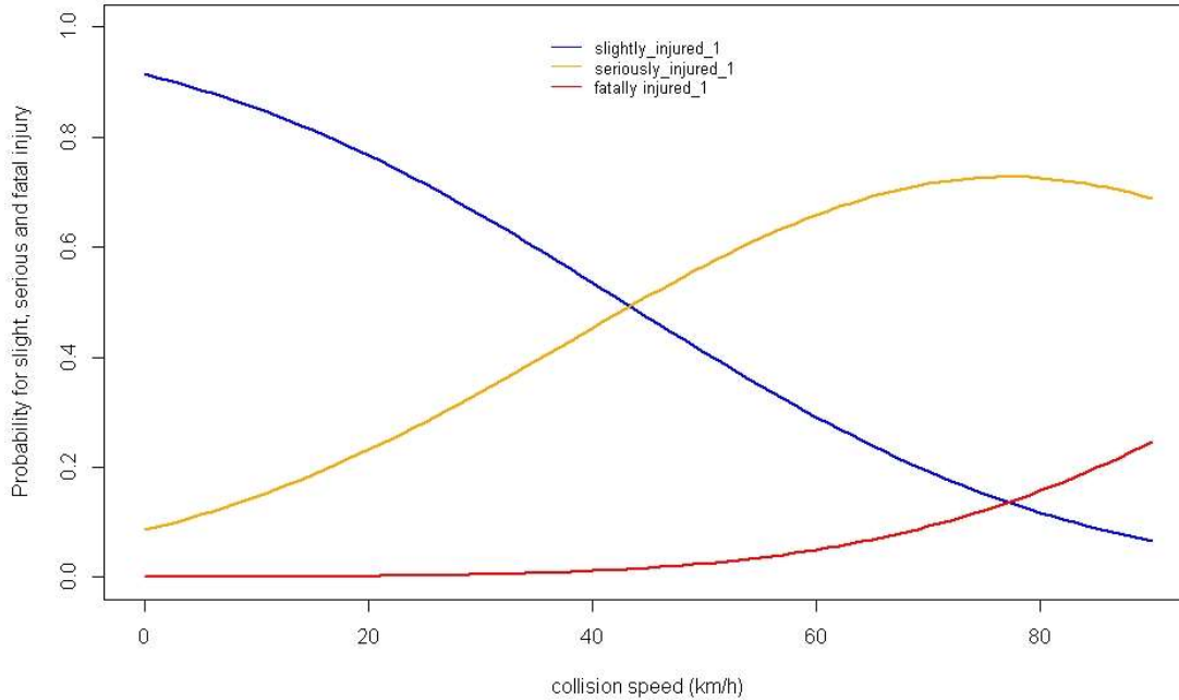
Figure 73: Probability of being slightly (blue), seriously (orange), and fatally (red) injured for cyclists in an accident with a car based on n=1,356 GIDAS cases identified as PROSPECT use-cases.
