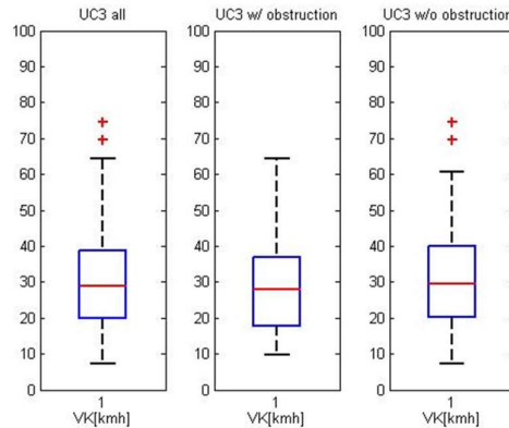
Figure 22: Box plots of the collision speed of the vehicle in UC_DEM_3
