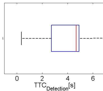
Figure 32: Box plot of detection times for UC_DEM_5 without view obstruction.
