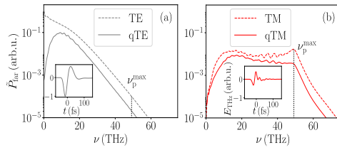
Fig. 2. Experimental THz spectra for qTE (a) and qTM (b) polarization (see text for details). Corresponding on-axis THz waveforms are shown as insets. The dashed lines specify the estimated maximum plasma frequency.
