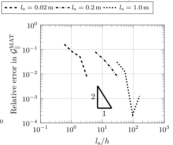
Figure 2.4: Convergence properties of the gradient-enhanced model for the problem of the single edge-cracked specimen. Case of “hard” boundary conditions, \epsilon^p = \mathbf{0} .
