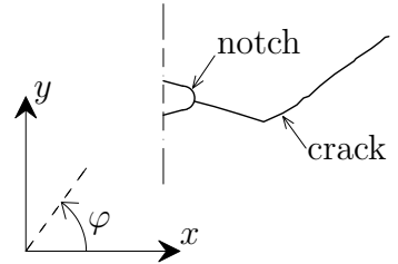
(c) Final crack configuration.
