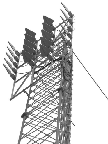
Fig. 1. Photo of the antenna array including the 20 log-periodic antennas. The outer two columns are vertically polarized and the inner two columns are horizontally polarized.
