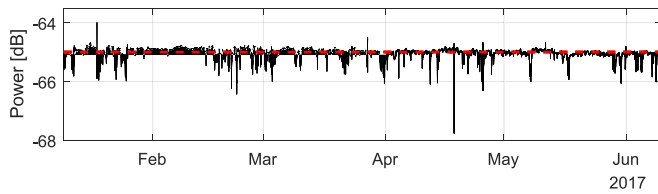
Fig. 6. Plot of the direct coupling peak power between the H-Tx and H-Rx antennas at P-band used for normalizing variations in the cable attenuation. The dashed red line shows the corresponding median for which the backscatter data in the channel are normalized for. The peaks coincide with rainfall events, likely due to a wet radome, and are treated as outliers.
