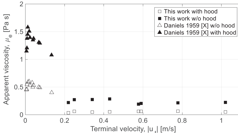
Figure 4. Apparent viscosity, \mu_e , calculated as proposed by Rees et al. [7] over the absolute terminal velocity, |u_t| , comparing data from this work and Daniels [3].
