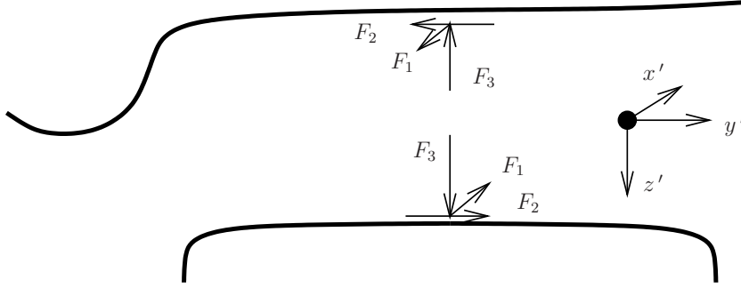
Figure 3.1: Moving reference frame of the interaction model.
