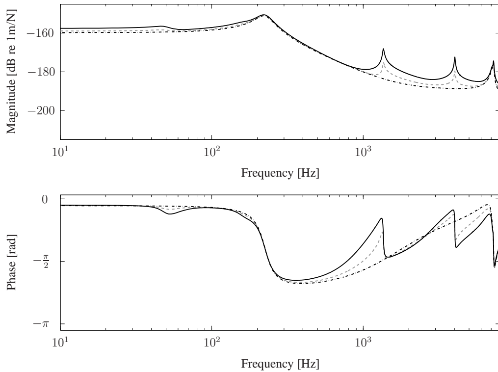
Figure 3.23: Comparisons of the magnitude and phase of the vertical point receptance calculated at different lateral positions on the rail head: Node 109 ( - \cdot - ), node 112 ( - - - , grey) and node 115 ( — ).
