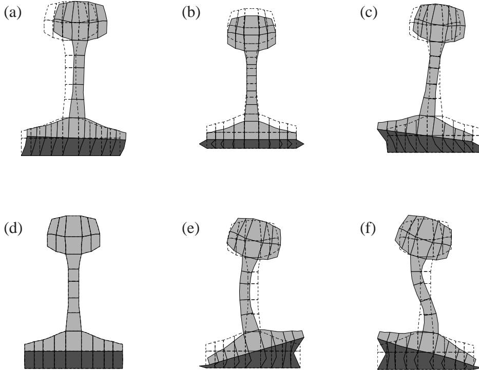
Figure 3.20: Wave shapes at k = 1 rad/m: (a) Lateral bending wave, (b) Vertical bending wave, (c) Torsional wave, (d) Longitudinal wave, (e) Web bending wave 1, (f) Web bending wave 2.
