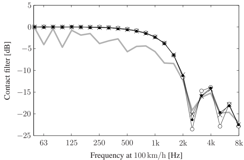
Figure 5.1: Dynamic wheel/rail interaction excited by roughness measured on a wheel with sinter block brakes (wheel 2 in Paper III): (a) average one third-octave band spectra of the vertical contact force and (b) average contact filter effect calculated from runs with seven different longitudinal roughness lines; contact model: — (thick grey line) 3D contact model, —×— 2D contact model, —●— Hertzian spring with roughness pre-filtering by the Winkler bedding, —○— Hertzian spring with roughness pre-filtering by averaging, --- Hertzian spring with no roughness pre-filtering.
