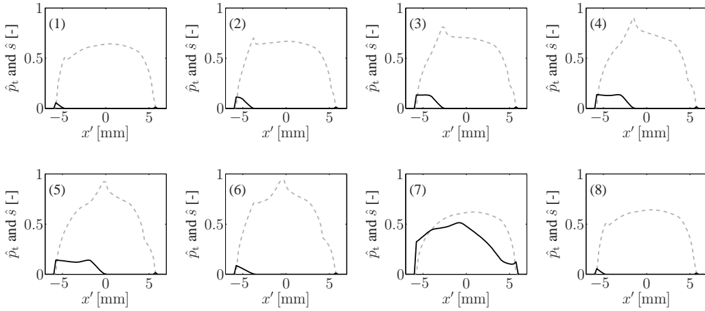
Figure 5.7: Time history corresponding to the time steps numbered in Figure 5.6 for the case \Delta x = 0.25 mm: --- (in grey) normalised tangential stress |p_t|/p_{\text{ref}} , — normalised local slip |s|/s_{\text{ref}} on line y' = 0 .
