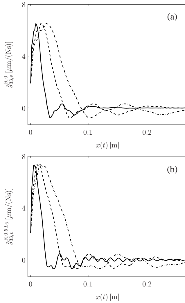
Figure 3.17: Moving Green's functions of the track for excitation (a) above a sleeper position, x_0 = 0 , and (b) at midspan between two sleeper positions, x_0 = 0.5 L_s : — v = 50 km/h, --- v = 100 km/h, -·- v = 150 km/h.
