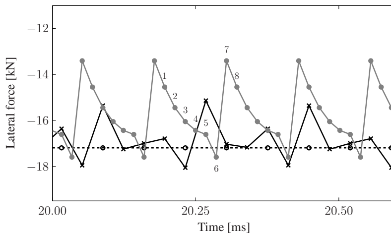
Figure 5.6: High-frequency oscillations under quasi-static conditions for different element lengths \Delta x : - \circ - 1 mm; - \times - 0.5 mm; - \bullet - 0.25 mm. Selected time steps are denoted by Arabic numerals.
