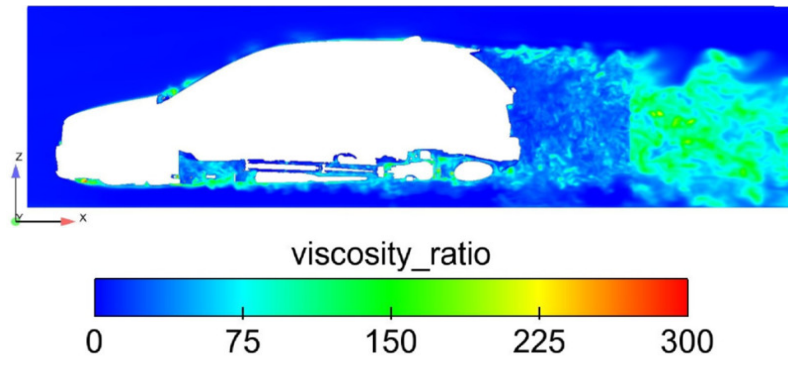
Fig. 9: DDES-performance analysis: \frac{\nu_t}{\nu} at symmetry plane
