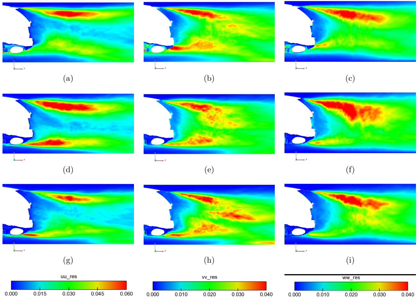
Fig. 22: Normalised turbulent stresses at the symmetry plane for \frac{\overline{u^2}}{U_\infty^2} (left), \frac{\overline{v^2}}{U_\infty^2} (middle) and \frac{\overline{w^2}}{U_\infty^2} (right): (a to c) Configuration 1, (d to f) Configuration 2 and (g to i) Configuration 3
