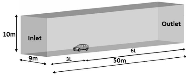
Fig. 4: Vehicle positioning in the numerical wind tunnel
