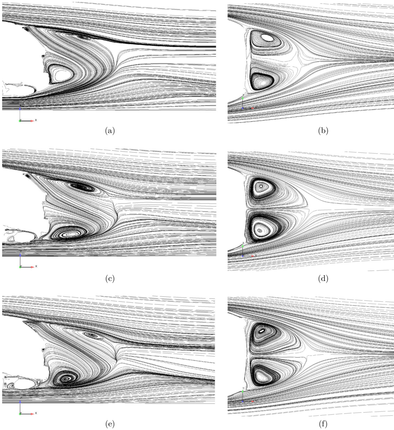
Fig. 18: Velocity streamlines in the wake behind vehicle for the symmetry plane (left) and a plane at z = 0.747m (right): (a-b) Configuration 1, (c-d) Configuration 2 and (e-f) Configuration 3
