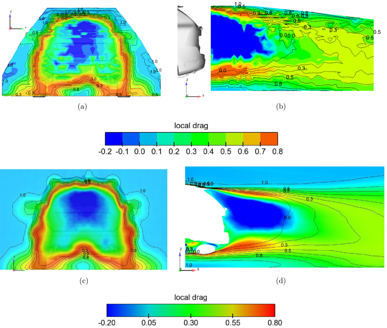
Fig. 17: Local drag superimposed with c_{p_{rot}} -contour lines: (a) Transverse plane WT, (b) Symmetry plane WT, (c) Transverse plane CFD and (d) Symmetry plane CFD
