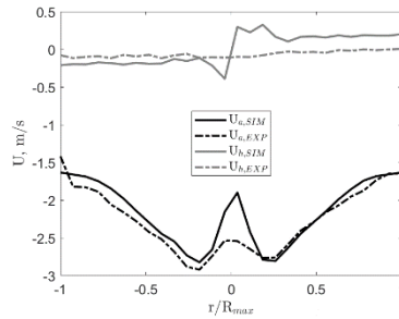
Figure 3: BEP experimental (EXP) and numerical (SIM) mean velocity profile comparisons at Line 1, where a = axial and h = horizontal. R_{max} is the largest radial position along the experimental line (i.e. extent of PIV plane, not draft tube wall).
